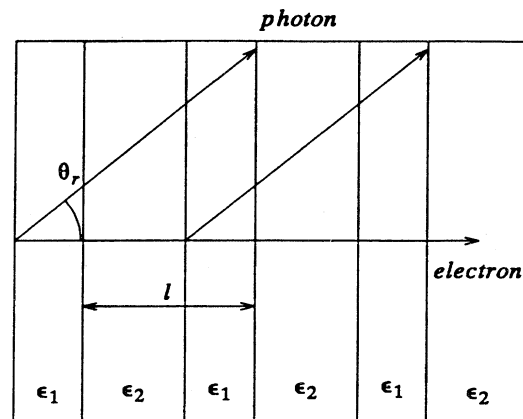
FIG. 1. The configuration of resonant TR.
